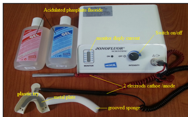
Figure (1): Iontophoresis device.
